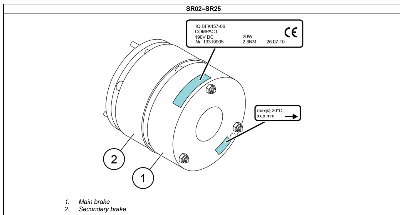
Figure 2. Double brake assembly – INTORQ brake
