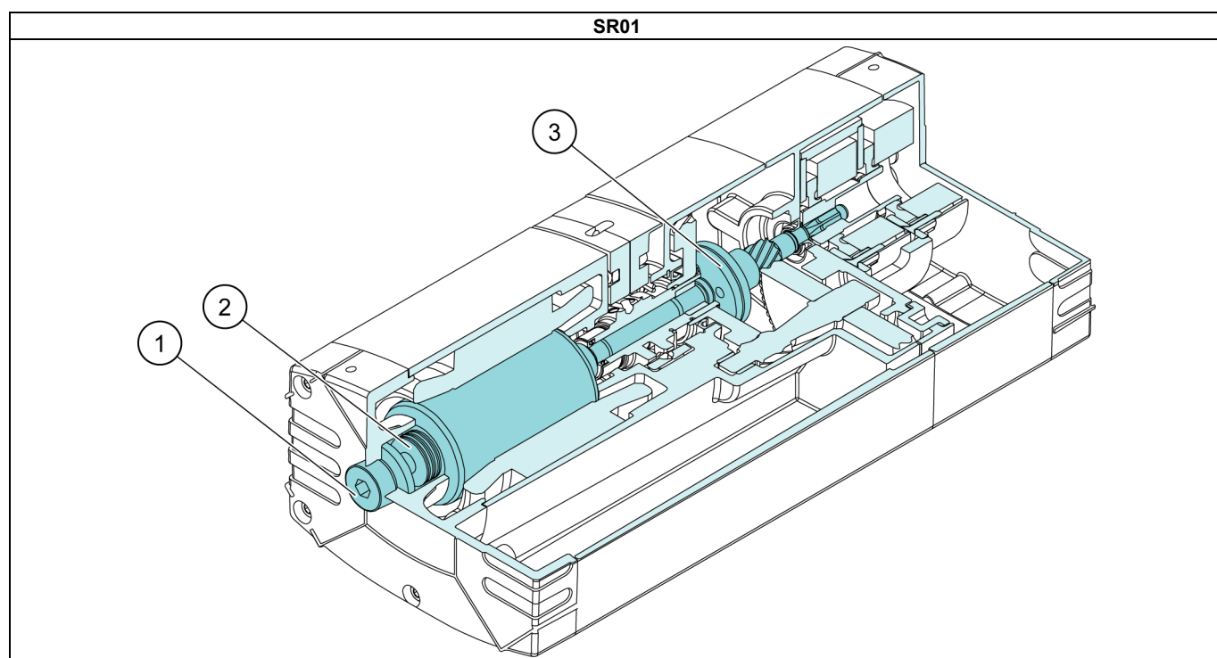
Figure 3. The clutch and the clutch adjustment principle of the SR01 hoist where the clutch adjustment is done from the motor side.
