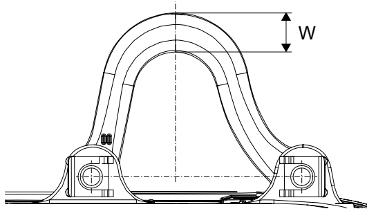
Abb. 17. Measuring wear on the suspension bracket (option)
