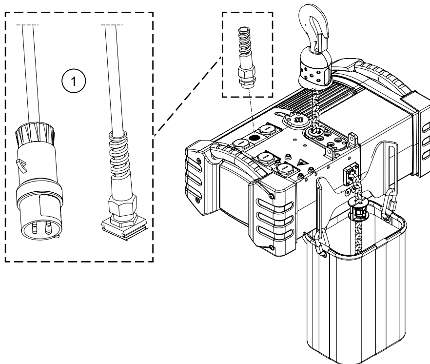
Abb. 12. Cable gland positions of the chain hoist configuration A
