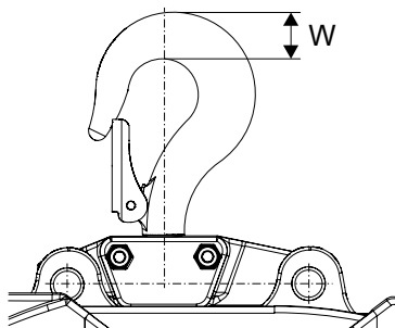
Abb. 16. Measuring wear on the rotating suspension hook
